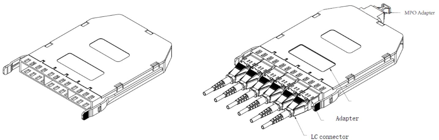
Figure 2. Giganet UHD-MTP/MPO Cassette Modules Base 8 Technical Drawing
