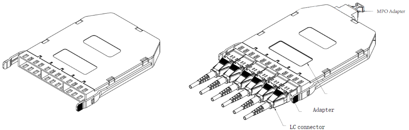
Figure 2. Giganet UHD-MTP/MPO Cassette Modules Base 12 (A and C) Technical Drawing
