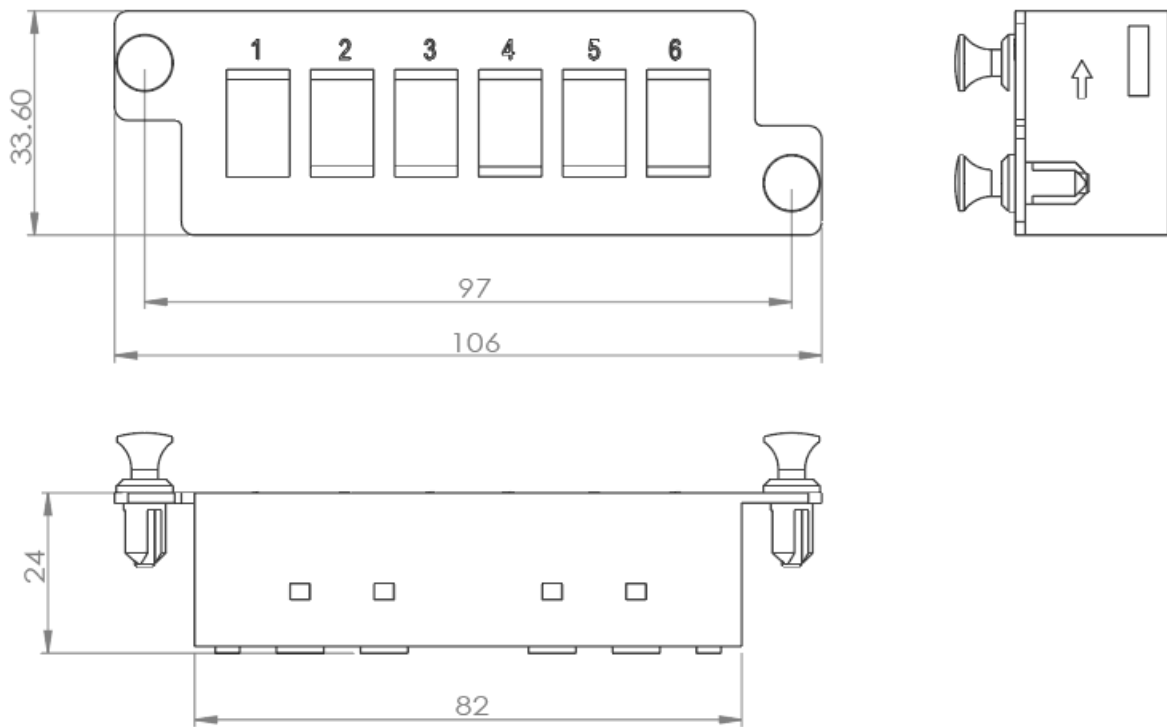
Figure 2. Gigaset HD-Pass through MTP/MPO Adapter Plates Technical Drawing
