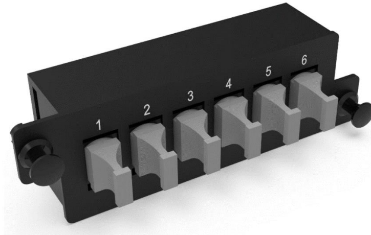
Figure 1. Giganet HD-Pass through MTP/MPO Adapter Plates
