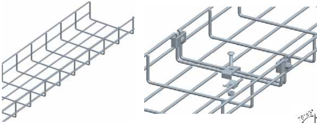
Giganet Wire Mesh (basket) Cable Tray
